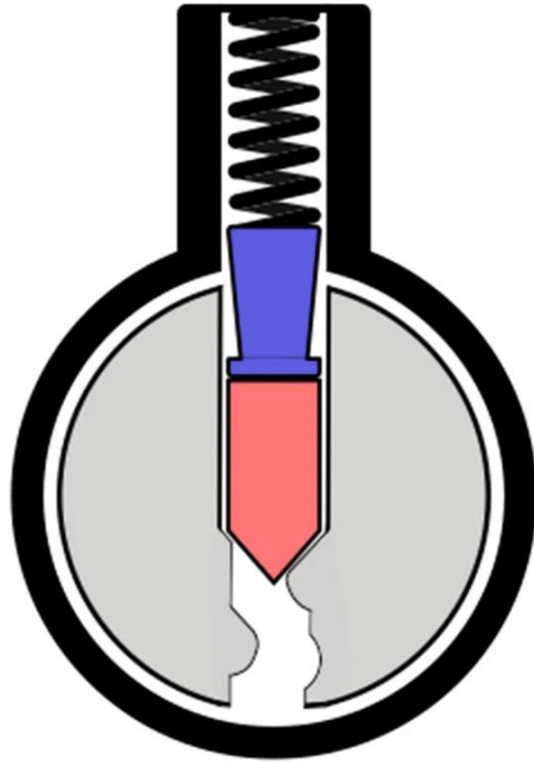
Mushroom Pin
