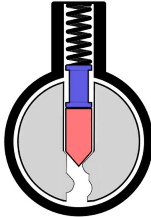
Spool Pin
