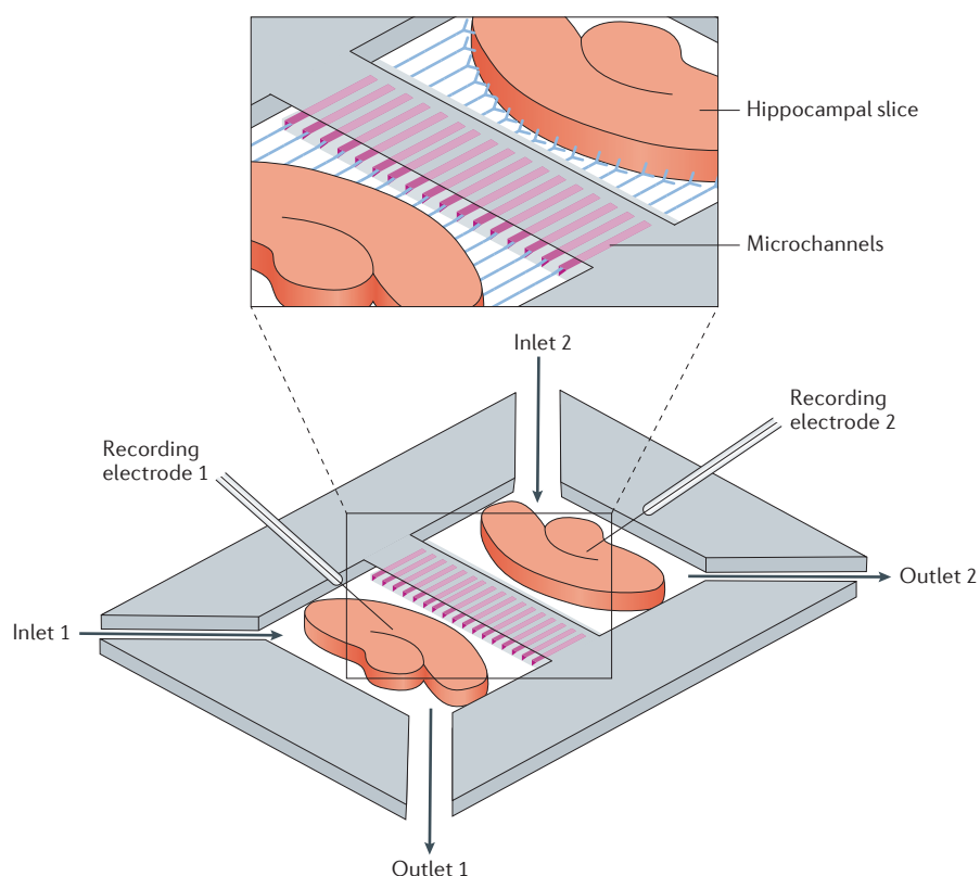
Figure 4 | Brain tissue-on-a-chip. Higher-order functionality of the nervous system can be studied in a microdevice that enables culture of two brain tissue slices in separate media formulations. The two tissue slices are allowed to communicate by synaptic connections formed through microchannels between the culture chambers. Electrodes incorporated into this system enable measurement of synchronous electrophysiological activity between the two brain slices. This design allows for selective pharmacological treatment of only one tissue slice and measurement of its effects across the synaptic connections.
